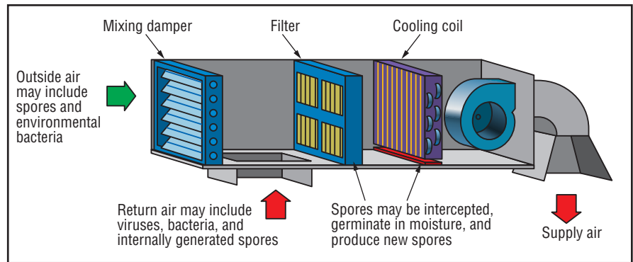
Figure 8. Sources and pathways of microbial contamination in a typical air handling unit.
